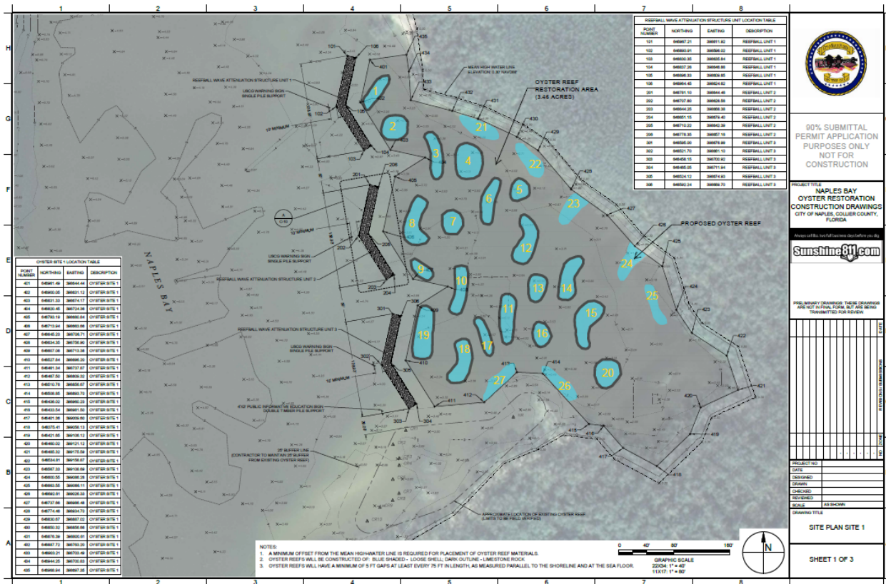
Figure 2. General Site 1 layout. Dark grey chevron shapes = ultra reef ball (or equivalent) placement. Blue areas = loose shell reefs. Dark grey around blue areas = limestone rock surrounding loose shell reefs. See Attachments B, D and E for details.
