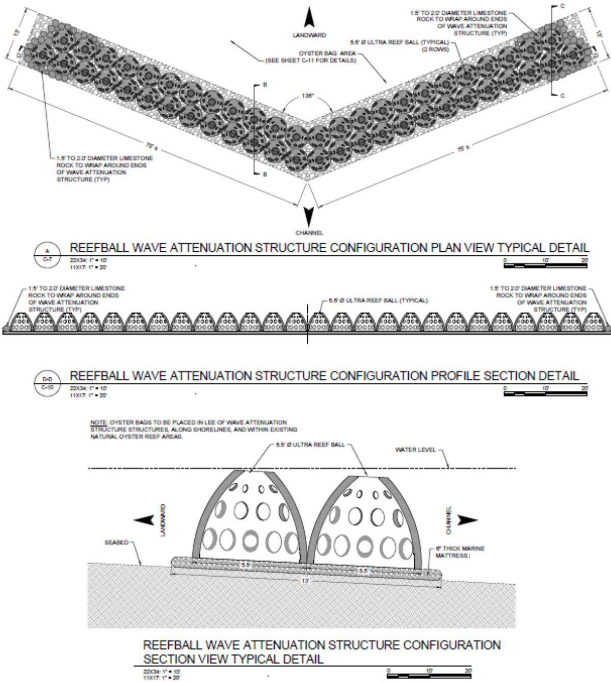
Figure 3. Basic design of wave attenuation reef ball structures (see Attachment E).
