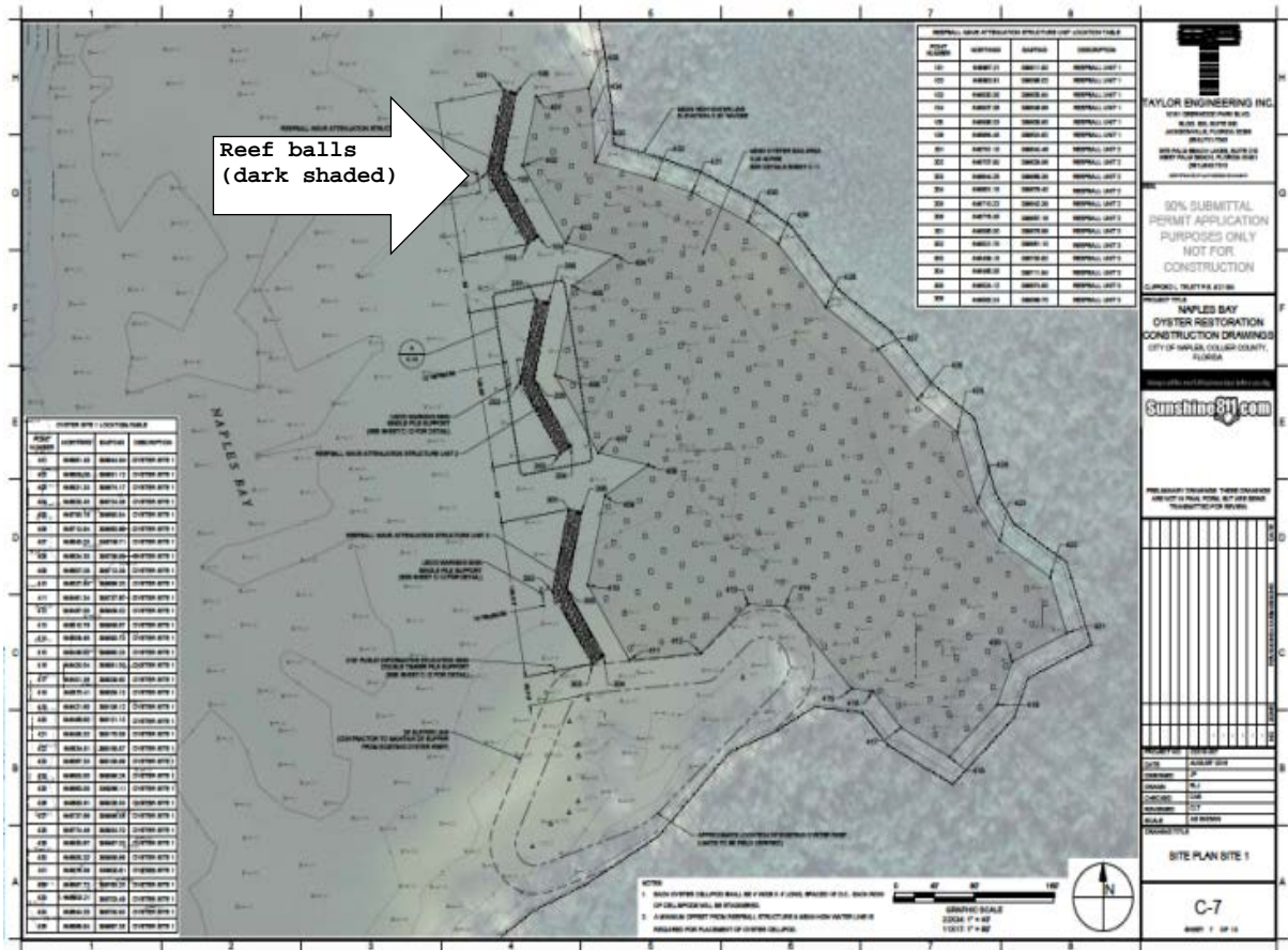
Figure 3. Reef ball placement design. Chevron-shaped reef ball structures will provide wave and storm surge attenuation and have a fifty (50) foot gap to allow for movement of water and marine organisms, such as managed fish species and manatees.
