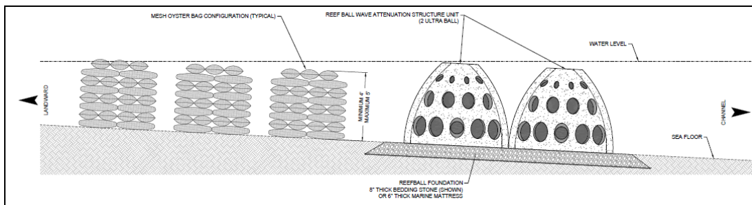
Figure 2. Basic design of reef ball structure and oyster reefs
