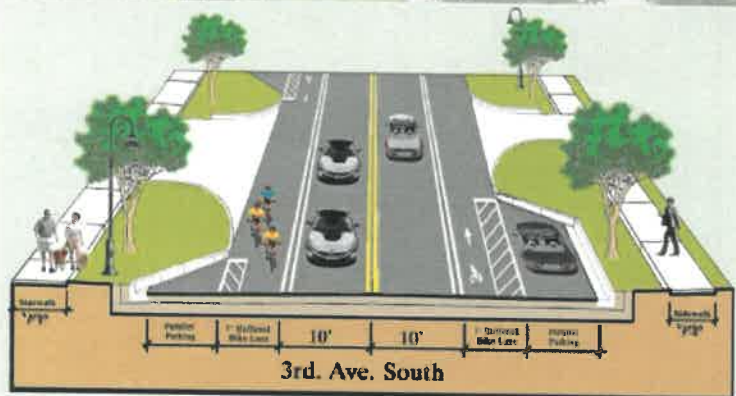
Conceptual Cross Section (80' right of way)
