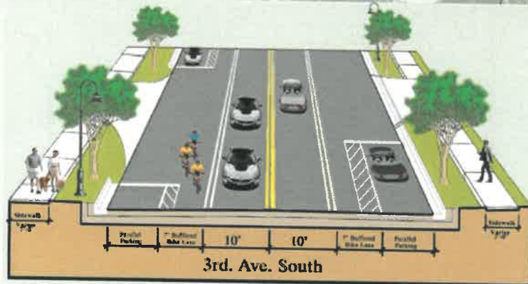
Conceptual Cross Section (80' right of way)
