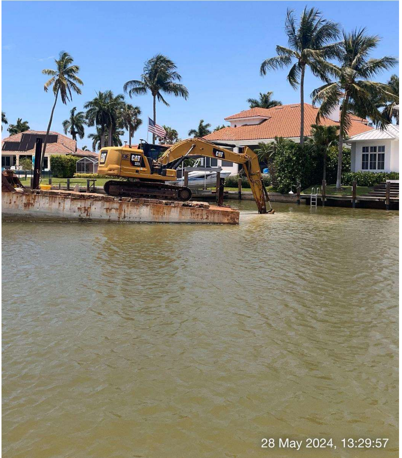
323 excavator grinding rock at station 13+60 in Canal A-A.
